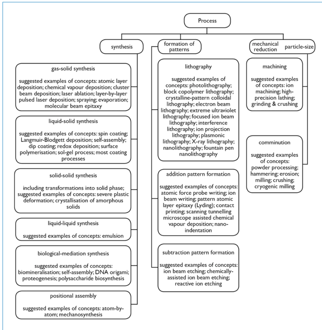
Figure 1. The various technologies and processes for synthesising nanomaterials (ISO / TR 12802: 2010).
