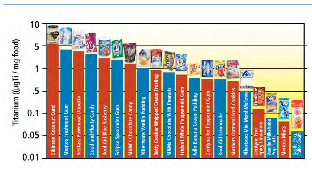
Figure 1. Titanium content (Ti in micrograms per milligram of weight of food) 8 .
